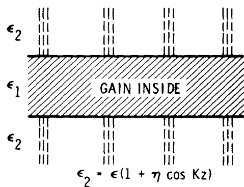
Fig. 2.1 Possible configurations for DFB lasers: (a) waveguide boundary perturbation, (b) periodic permittivity inside the waveguide, (c) periodic permittivity in the substrate. The active medium can be either in the waveguide or in the substrate.
