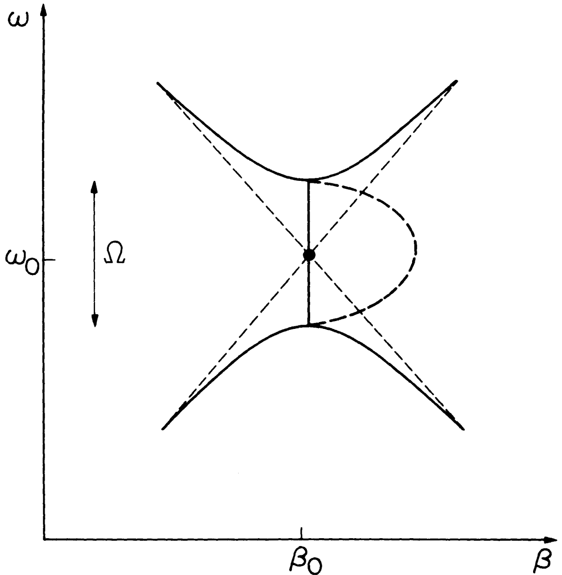
Fig. 2.4 \omega - \beta diagram near an interaction region. The solution for \beta is complex. The dashed curve is the imaginary part of \beta and the solid curve is the real part of \beta .
