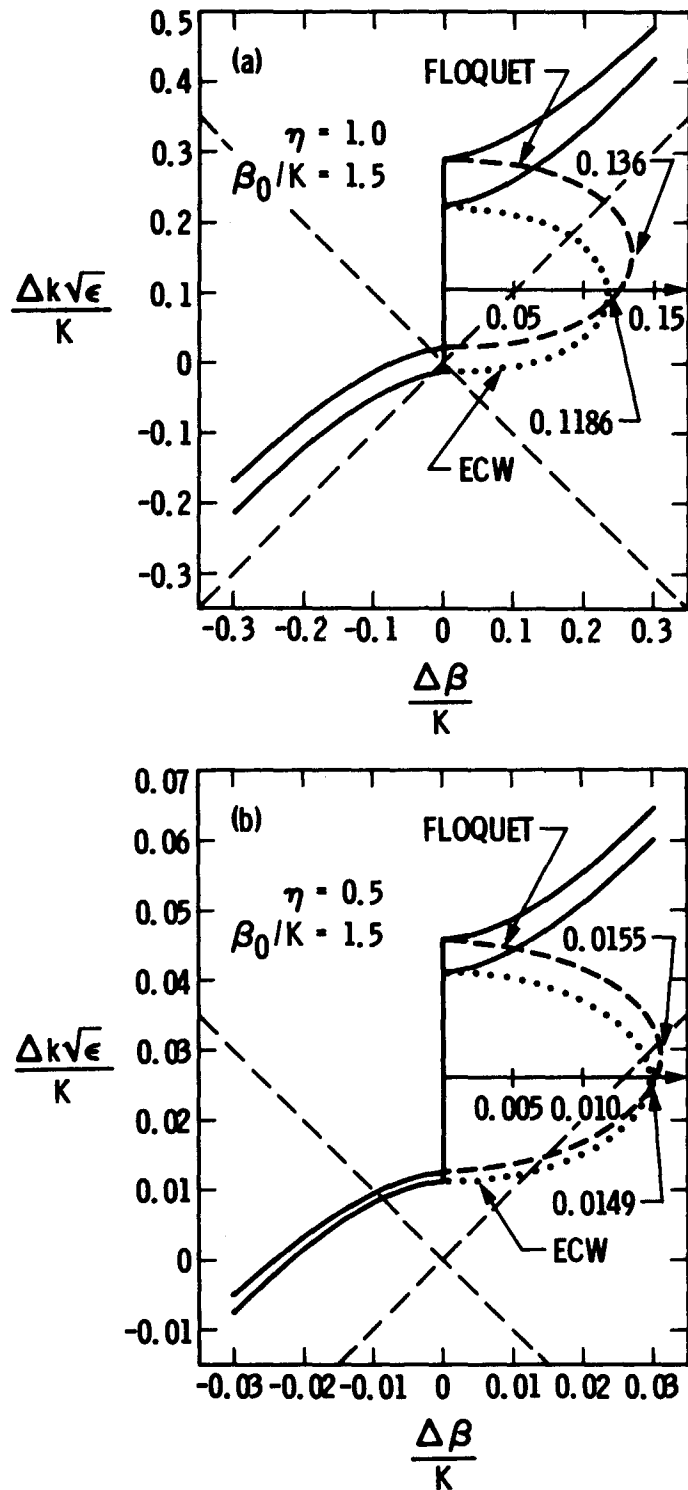
Fig. 5.6 Brillouin diagram at third Bragg order for a) \eta = 1.0 and b) \eta = 0.5 showing Floquet and ECW results. Imaginary \Delta\beta/K values are the elliptical curves with separate scale.
