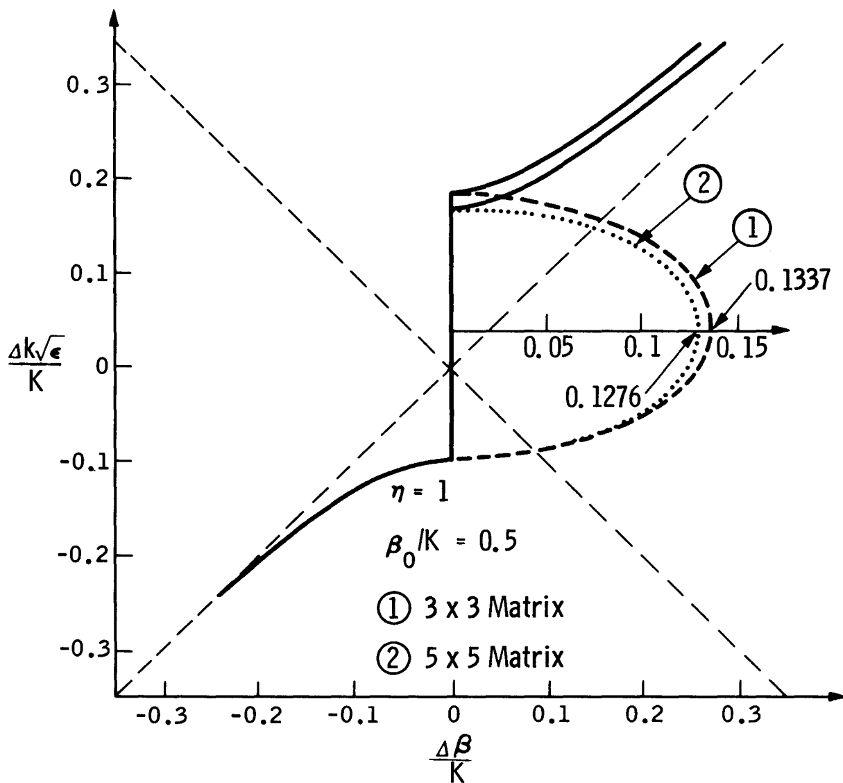
Fig. 2.10 The effect of limiting space harmonics in the Brillouin diagram using Floquet theory at the first Bragg interaction.
