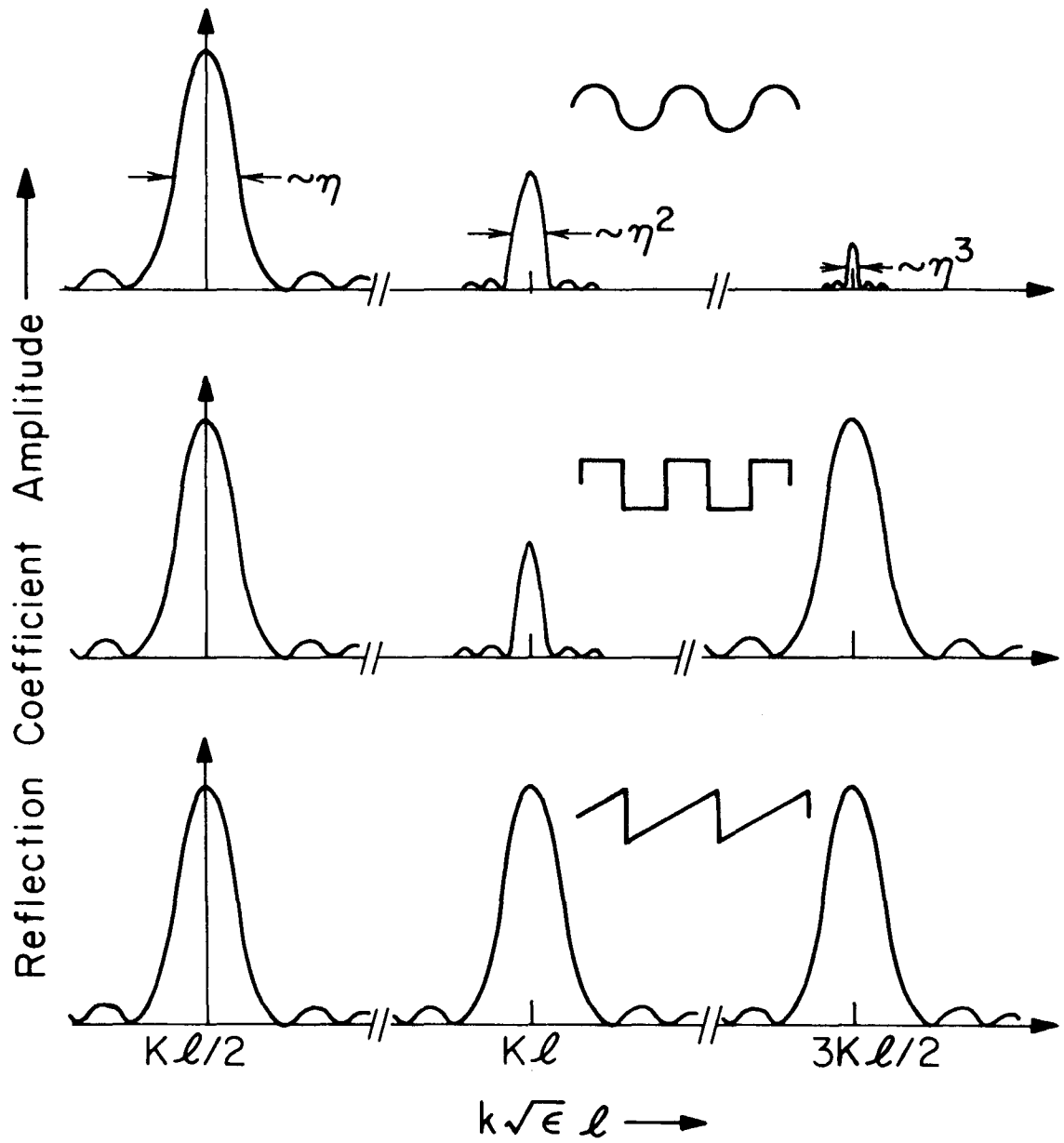
Fig. 6.6 Sketches of reflection coefficient amplitude for \chi l \sim 0.5 for a) sinusoidal, b) square-wave and c) sawtooth-wave periodicities. In all cases the boundary effects are neglected. Note small reflection at N^{\text{th}} Bragg order when f_N = 0 . The bandgap shift is too small to observe on this scale.
