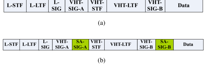
Fig. 2: Frame format: (a) VHT mode in IEEE 802.11ac. (b) the proposed SA-VHT mode.
