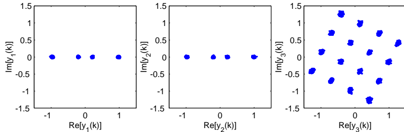
Fig. 2. Output signal constellations obtained by (8)–(9) for a source clustering task in wireless communications.
