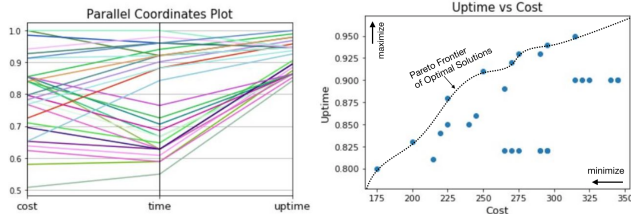
Fig. 5. Plot of candidate solutions - cost and time functions are scaled.
