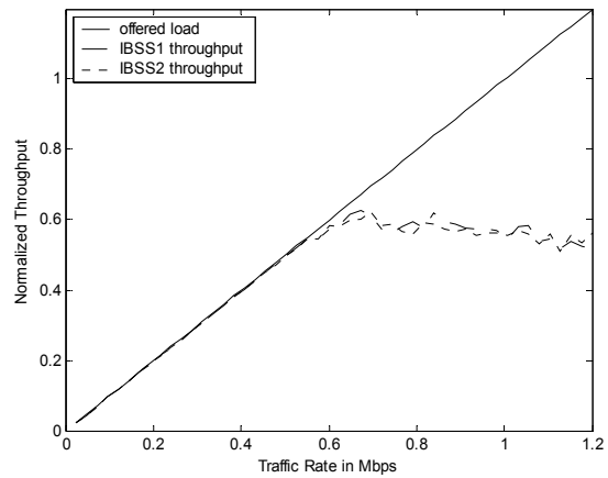
Fig. 6 Algorithm throughput
