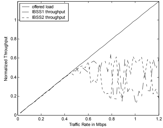
Fig. 5 Overlapping IBSSs throughput
