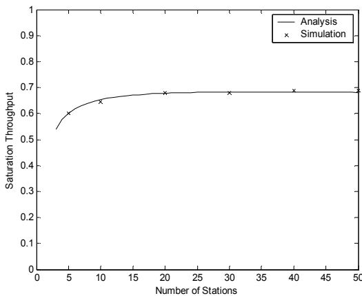
Fig. 9 Analysis versus Simulation
