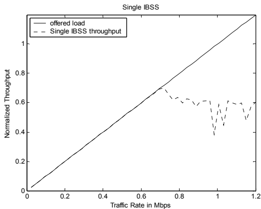
Fig. 4 Single IBSS throughput
